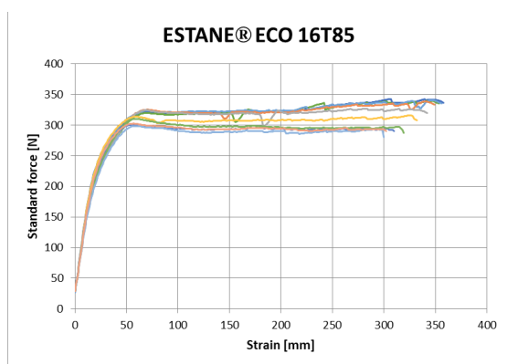
Figure 3. Adhesion strength traces of ESTANE® ECO 16T85 overmolded onto Tritan™ TX1501HF. The average adhesion strength value calculated from this data was found to be 311 N.
