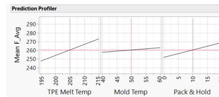
Figure 2. Average force average plotted against each parameter's respective values. Plot #1 displays an increase in average force as TPE Melt Temperature increases, Plot #2 displays an increase in average force as Mold Temperature increases, and Plot #3 displays an increase in average force as Pack and Hold Time increases.
