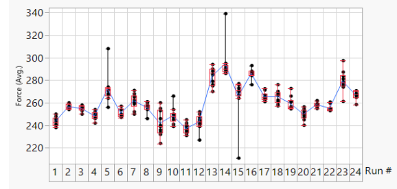
Figure 1. Average force values (blue line) plotted vs DoE run number. Median force values, which remove the effect of outliers, are displayed by the middle line in the box plot.
