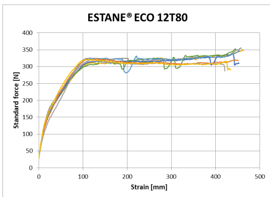
Figure 4. Adhesion strength traces of ESTANE® ECO 12T80 overmolded onto Tritan™ TX1501HF. The average adhesion strength value calculated from this data was found to be 316 N.
