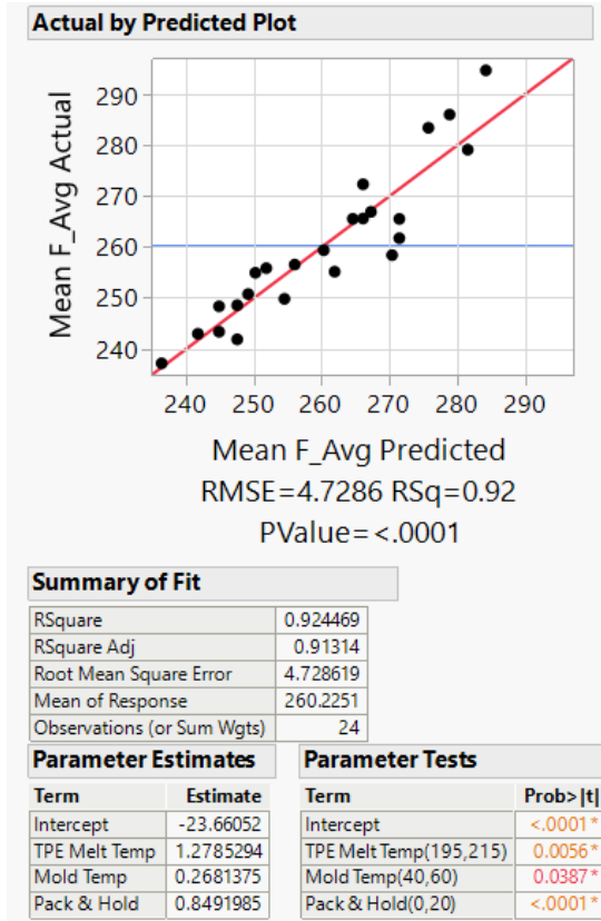
Figure A1. The experimental values plotted vs the model's predicted value show good agreement. Specifically, the R-Square and Adjusted R-Squared statistics are 0.92 and 0.91, respectively. The parameter tests table shows that TPE Melt Temperature, Mold Temperature, and Pack and Hold Time are statistically significant at the 95% confidence level. The effect of Injection Speed was not significant and was removed from the model. The parameter estimates can be used to predict the average of the average force within the ranges of the process factors studied.
