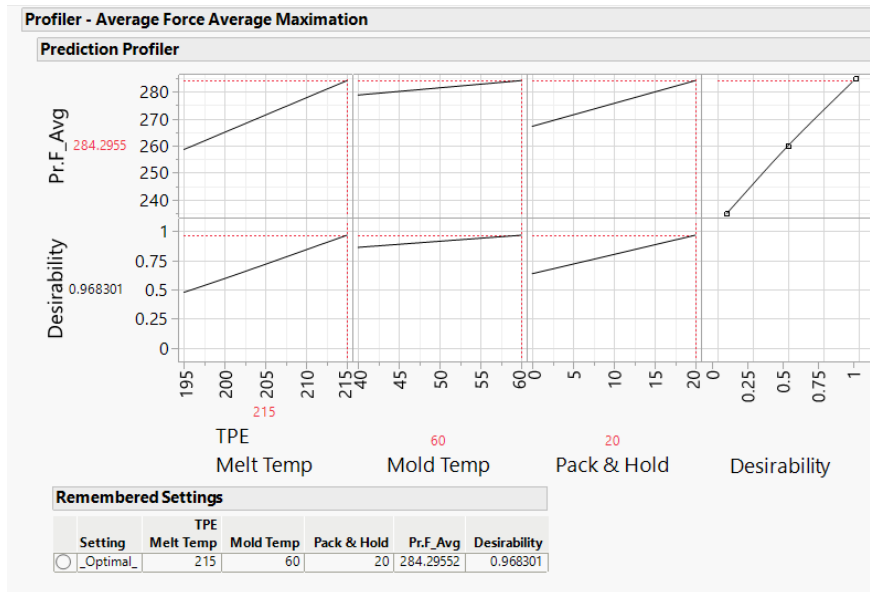
Figure A2. The Profiler shows that optimizing the processing settings to generate a maximum adhesion force predicts a value of 284 N. In order to obtain this value, all parameter (TPE Melt Temp, Mold Temp, and Pack and Hold Time) should be maximized.
