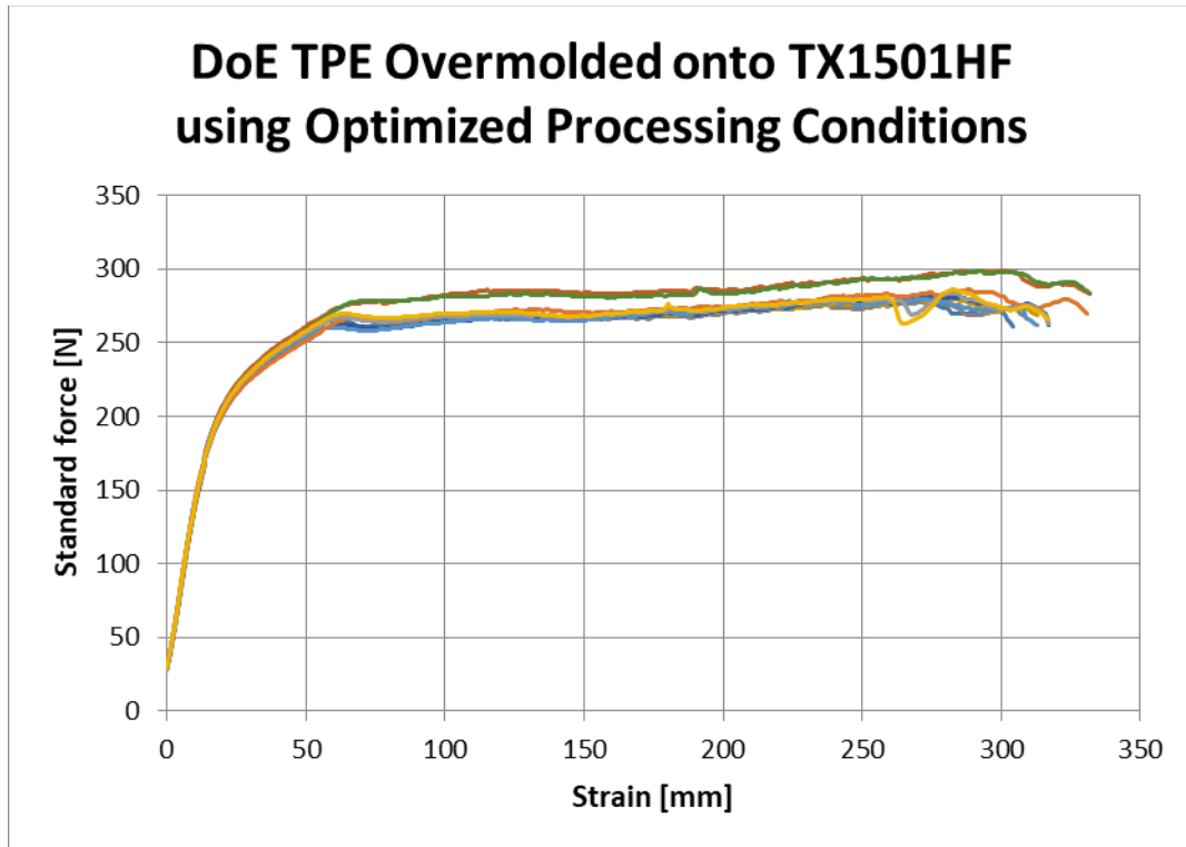
Figure A3. Adhesion strength traces of the DoE TPE (not identified) overmolded onto Tritan™ TX1501HF using the optimized settings identified by the DoE profiler. The average adhesion strength value calculated from this data was found to be 274 N, which is within one standard deviation of the adhesion strength value predicted by the profiler.
