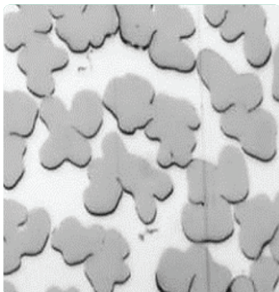
Naia™ Renew fiber popcorn cross section
