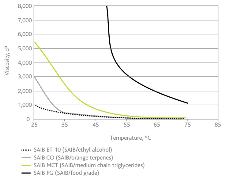
Figure 1. Viscosity behavior of Sustane SAIB food grade, kosher and blended products
